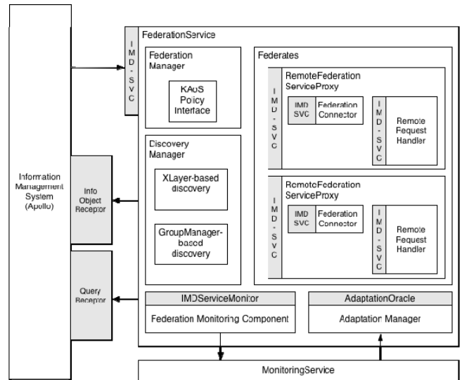
Figure 3: Federation Interfaces and Federation Service Architecture
