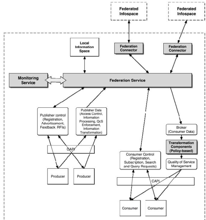
Figure 2: Architecture for Federation
