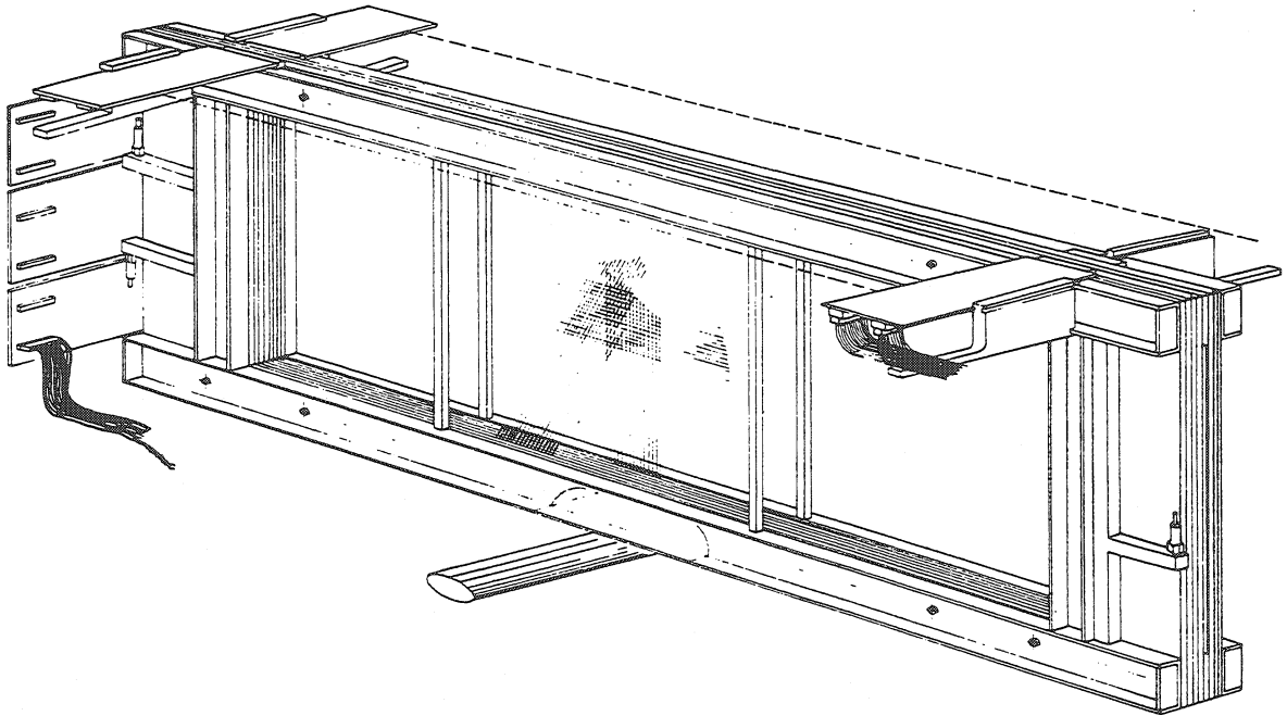
Fig. 79 Schematic view of an assembled three-coordinate medium-size multiwire proportional chamber 55) .
