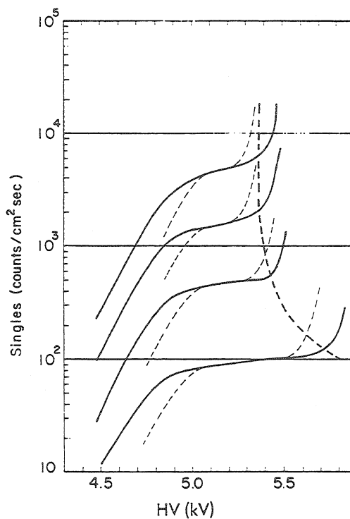
Fig. 77 Ageing effect in a chamber operating with organic gas mixtures (argon-isobutane 70-30) 33 ). The singles counting rate has been measured in a chamber for increasing intensities of ^{55}\text{Fe} X-rays, as a function of high voltage, before and after an irradiation of about 10^7 counts/cm 2 . After the irradiation, the average pulse height is reduced, for a given voltage, and the discharge knee appears at lower voltages.
