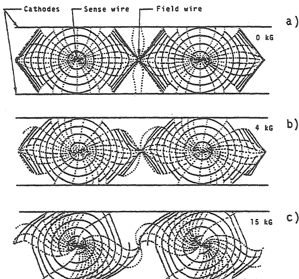
Fig. 96 Computed electron trajectories in a chamber like the one of Fig. 86, for several values of the magnetic field, parallel to the wires 78)
