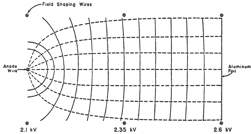
Fig. 90 The drift chambers developed at Fermilab with a thin aluminium foil separating adjacent cells 76) .
