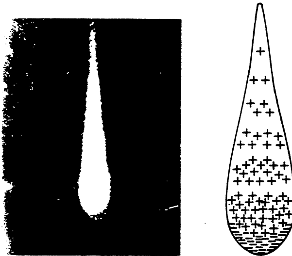
Fig. 46 Drop-like shape of an avalanche, showing the positive ions left behind the fast electron front. The photograph shows the actual avalanche shape, as made visible in a cloud chamber by droplets condensing around ions 18) .
