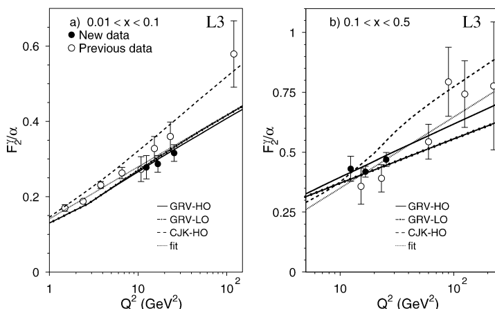
Fig. 7. Evolution of the photon structure function F_2^\gamma/\alpha as a function of Q^2 for two x intervals. The results of a fit to the data of the function a + b(\ln Q^2/\text{GeV}^2) are shown together with the predictions of the higher-order parton density functions GRV and CJK as well as the leading-order predictions of GRV.
