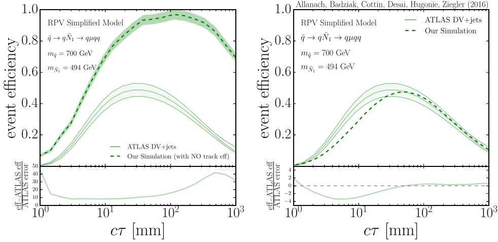
Figure 82. Validation of the DV + jets search for the ATLAS benchmark of a simplified RPV model with a 700 GeV squark decaying to a neutralino, \tilde{q} \rightarrow q(\tilde{N}_1 \rightarrow \mu\bar{u}d) . Left: without any tracking efficiency. Right: with a tracking efficiency function given by equation (6.11), taken from [206].
