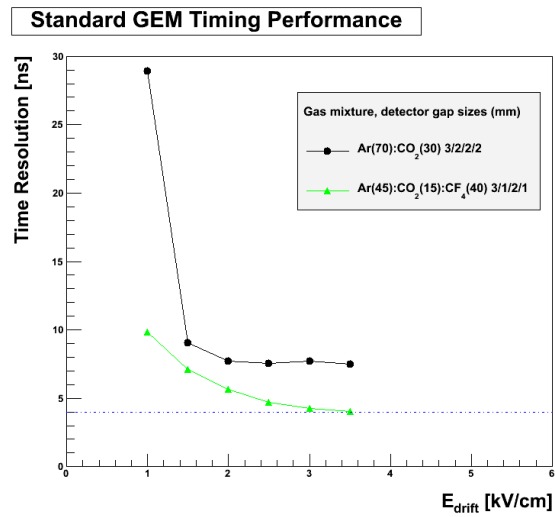
Fig. 9. Detector timing resolution as function of the induction (top) and drift (bottom) field for the standard triple-GEM with different gas mixtures and gap size configurations.
