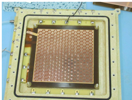
Fig. 3. The triple-GEM prototype with honeycomb spacers.
