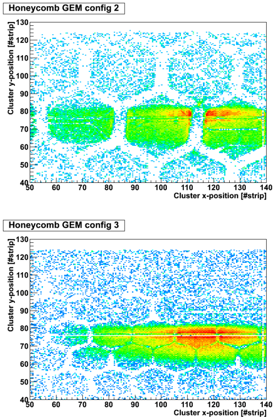
Fig. 12. Reconstructed cluster positions in the subregions near the beam spot of two different honeycomb triple-GEM configurations.
