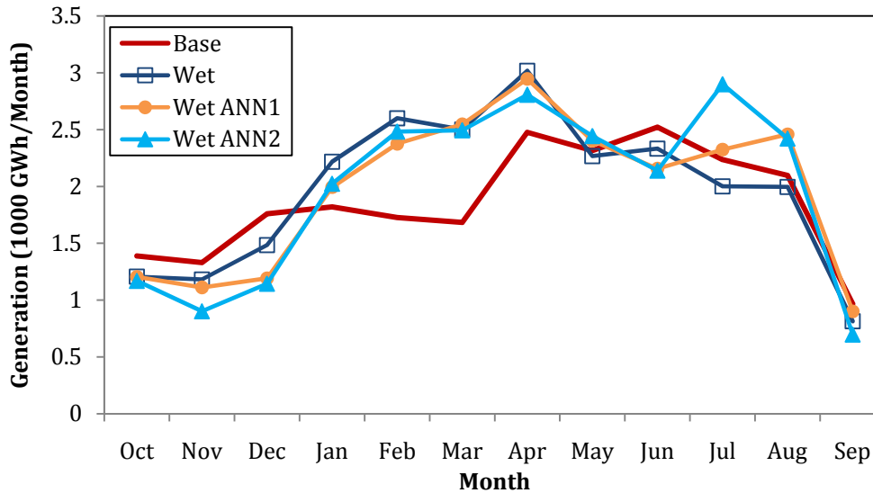
Figure 21: Average Monthly Generation (1985–1998) under Dry (Top) and Wet (Bottom) Warming Scenarios, Considering the Warming Effects on Hydropower Supply and Demand Simultaneously (Future Energy Pricing Is Forecasted Using ANNs – ANN1: Monthly Based Model; ANN2: Annually Based Model Calibrated on Normal Prices)
