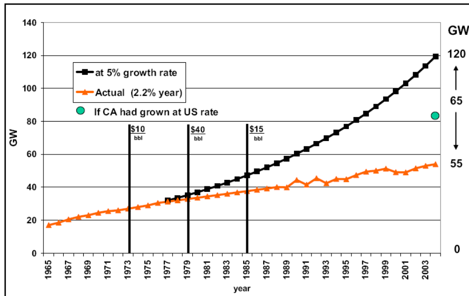
Figure 4: California Peak Electricity Demand, 1965–2004
