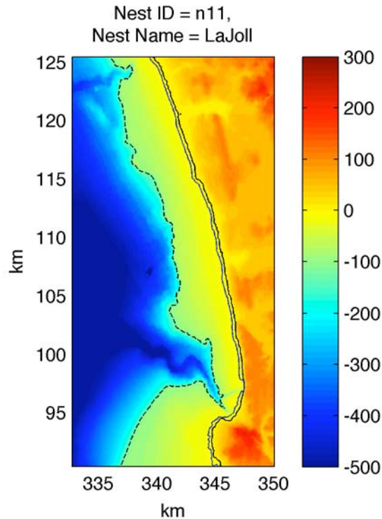
Figure 1-2. Bathymetry of five detailed nested regions used in this study. Nests are referred to as Santa Barbara (SntBrb), Santa Monica Bay (SntMnc), San Pedro (SnPdro), Dana Point (DanaPt), and La Jolla (LaJoll), respectively. In each nest view, the solid black line shows modern, mean sea level shoreline, the solid blue line shows the location of the 5-meter isobath, and the dashed black line shows the location of the 120-meter isobath, considered to be the edge of the continental shelf. Color bars correspond bathymetric elevation in meters above/below mean sea level.
