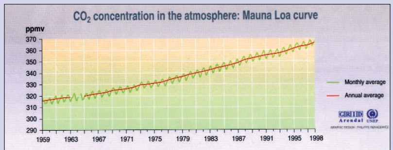
Figure 8. Collected with the intent of better understanding the carbon cycle, Charles Keeling's Mauna Loa Curve provides a remarkable set of data on atmospheric carbon dioxide ( \text{CO}_2 ) concentrations that are now an integral part of climate change science. The steady upward trend shows increases in annual average \text{CO}_2 concentrations due to fossil fuel emissions, and the saw-tooth line shows the yearly cycle in \text{CO}_2 concentrations due to seasonal changes in Northern Hemisphere vegetation. Source: Scripps Institution of Oceanography, University of California, 1998.
