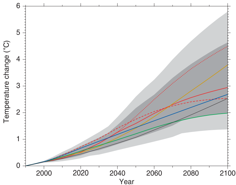
Figure 10. Climate models are often used to help inform policy decisions. The figure shows the projected global mean temperature change for several different scenarios of future emissions based on assumptions of future population growth, economic development, life style choices, technological change, and availability of energy alternatives. Each line represents the average of many different models run for the same scenario. Each model incorporates different assumptions to handle uncertainties in our understanding of natural climate processes. Source: Intergovernmental Panel on Climate Change (IPCC)
