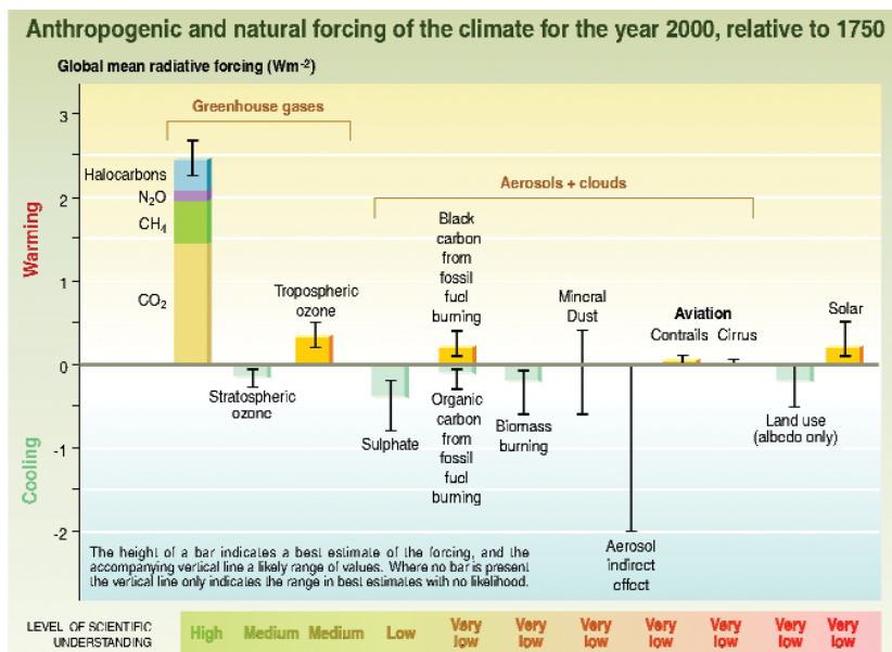
Figure 5. Various climate drivers, or radiative forcings, act to either warm or cool the Earth. Positive forcings, such as those due to greenhouse gases, tend to warm the Earth, while negative forcings, such as aerosols from industrial processes or volcanic eruptions, tend on average to cool it. If positive and negative forcings remained in balance, there would be no warming or cooling. Source: Intergovernmental Panel on Climate Change.
