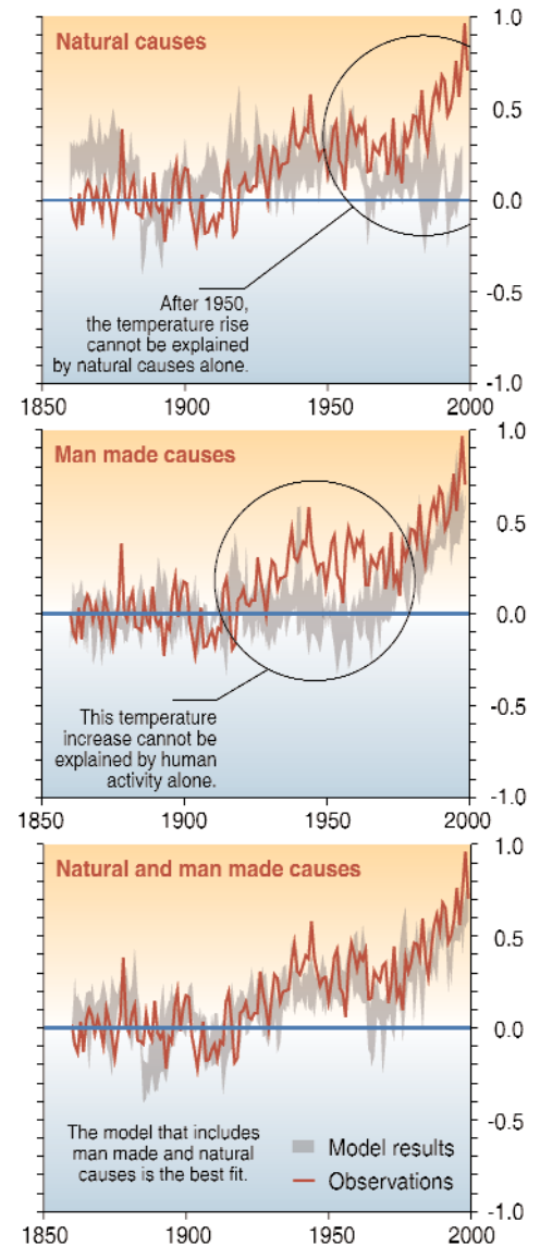
Temperature anomalies in ^{\circ}\text{C}
