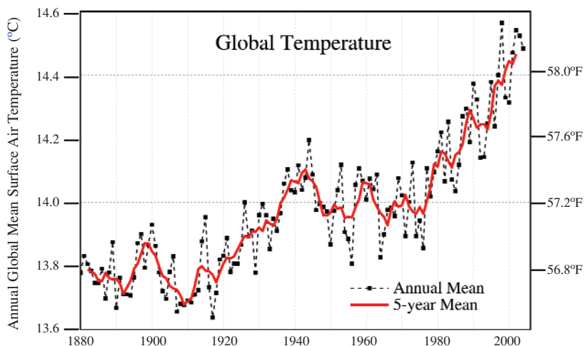
Figure 2. Global annual-mean surface air temperature has increased by 1.4° F (0.7°C) since the early 20th century, with about 0.9°F (0.5°C) of the increase occurring since 1978. Figure courtesy of Goddard Institute for Space Studies.
