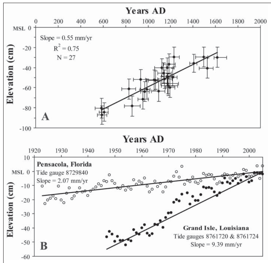
Fig. 2. (a) Long-term trend of relative sea level rise for the period 600 to 1600 A.D. The data set contains 27 sea level index points and records approximately 55 centimeters of relative sea level rise. Data points (with age and elevation errors) are defined by the median of calibrated ^{14}\text{C} ages plus elevation of the center of basal peat samples dated. Two subsamples were dated for each sample, and all but four index points were obtained by calculating a weighted mean of two ^{14}\text{C} ages. Only one sample provided a stratigraphically reversed age and was rejected. MSL is present mean sea level. (b) Trend of relative sea level rise for two selected tide gauges normalized to present mean sea level. Data were obtained from the U.S. National Oceanic and Atmospheric Administration's National Oceanic Service Center for Operational Oceanographic Products and Services. The locations of the tide gauges are shown in Figure 1.
