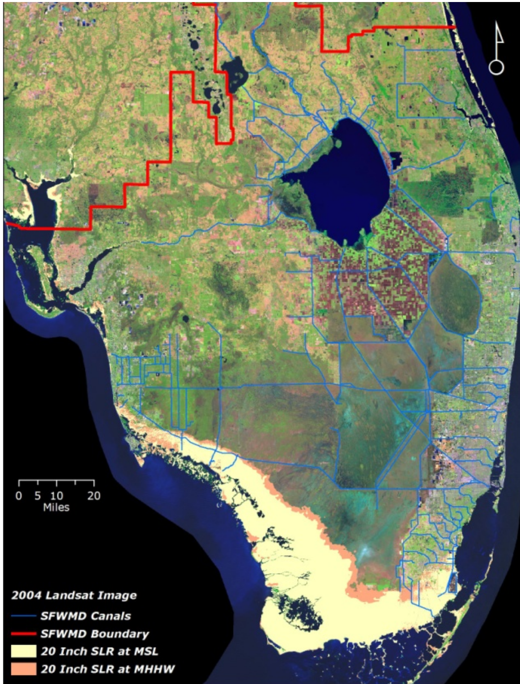
Figure 6. Possible permanent inundation and/or increased flooding of land within the District with a sea level rise (SLR) of 20 inches, the upper bound of projections for this paper, at mean sea level (MSL) and mean higher high water (MHHW). Tidal station data is averaged across the District and related to NAVD88. (Map produced by the SFWMD.)
