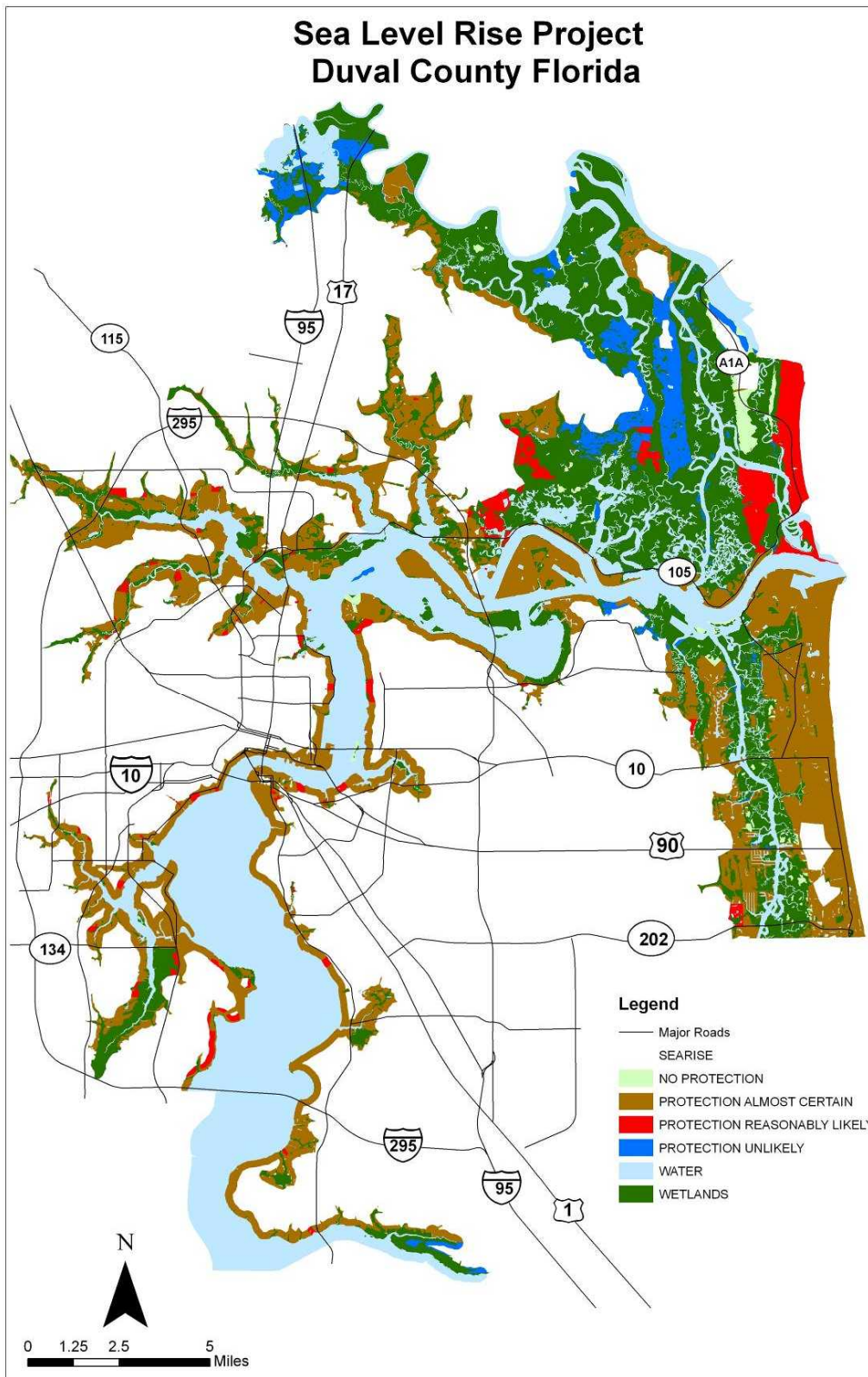
Map 2: Duval County: Likelihood of Shore Protection
