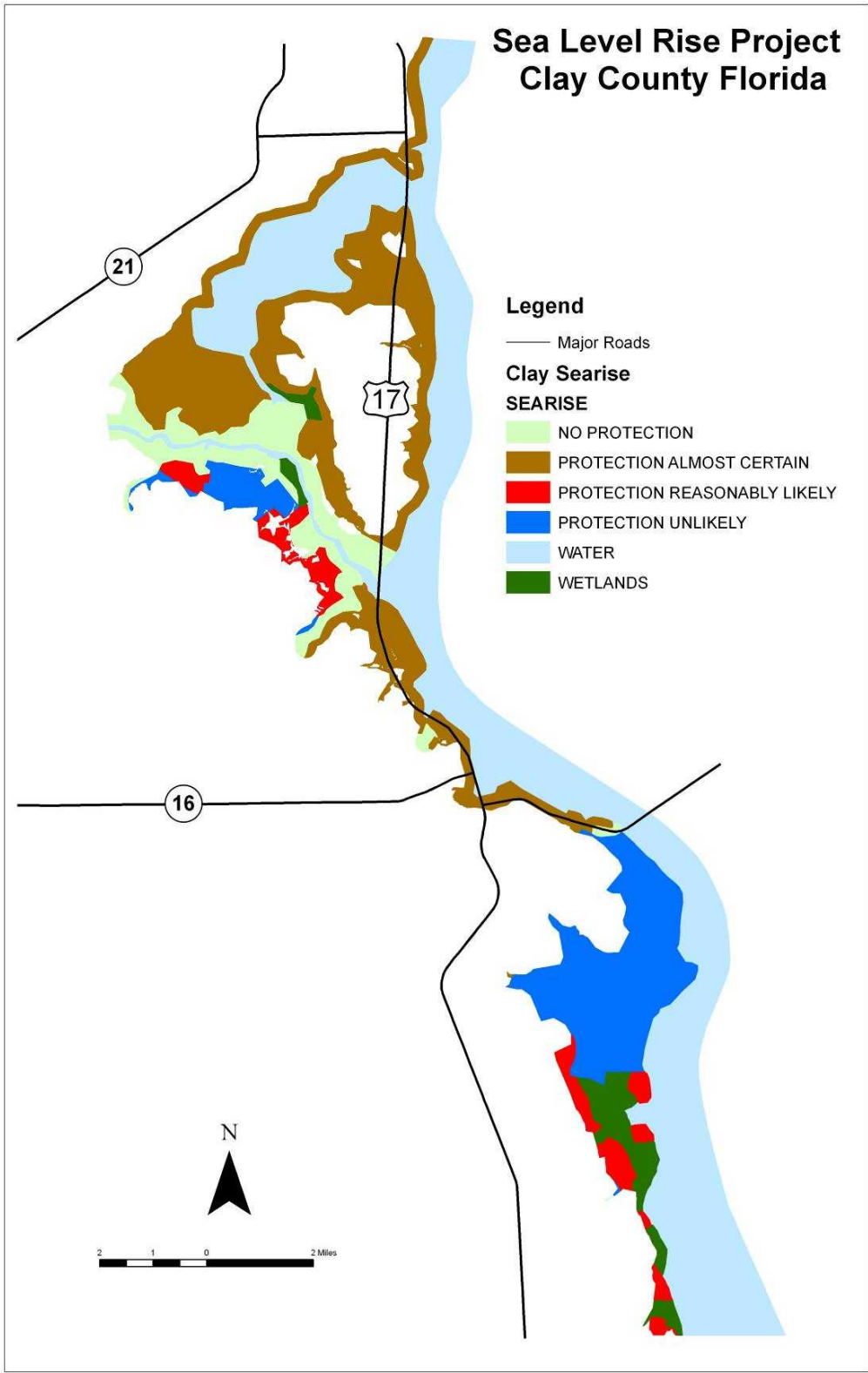
Map 5: Clay County: Likelihood of Shore Protection
