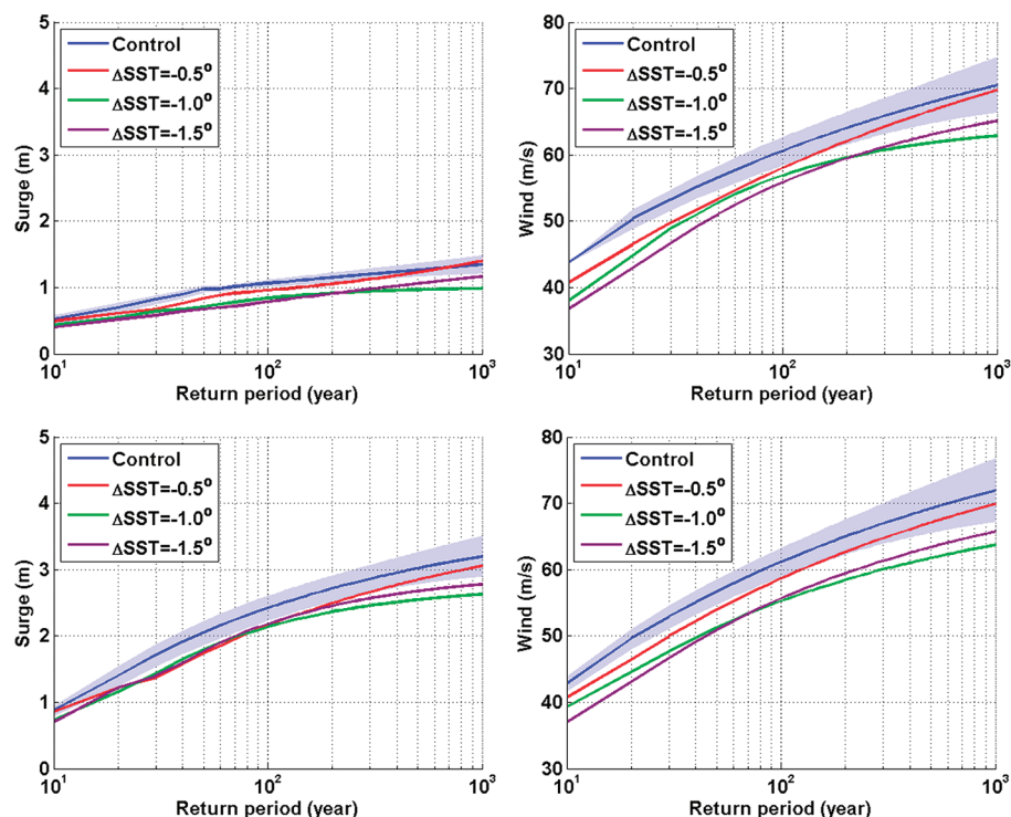
Figure 2. Storm surge and wind return level curves for Region 1 (top) and 2 (bottom). Legend indicates SST reduction from control. The shading shows the 90% confidence interval for the control scenario.
