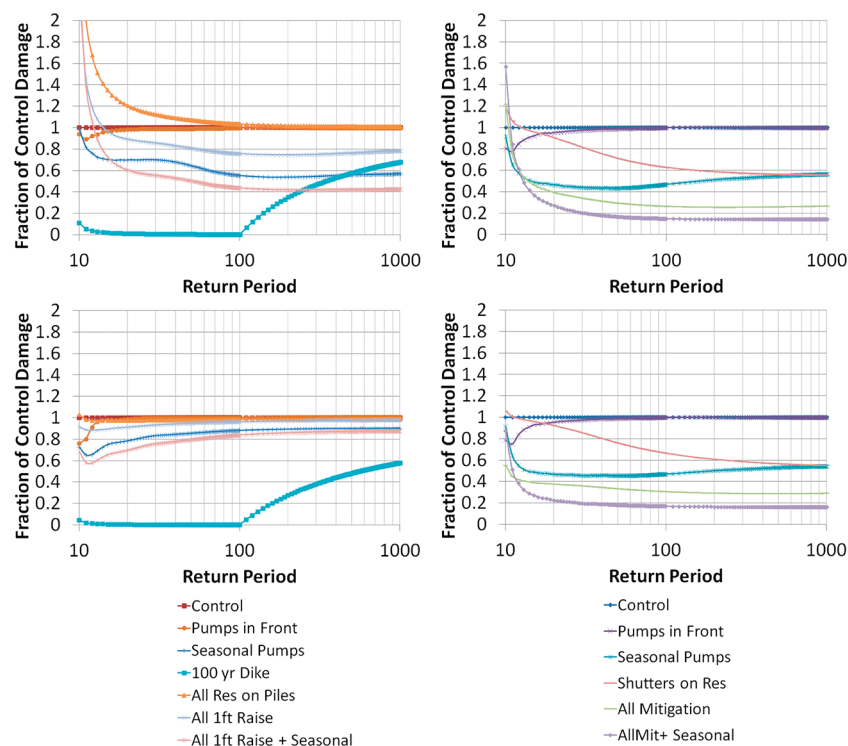
Figure 4. Seasonal expected fraction of control damage for scenarios combating storm surge (left) and wind damages (right) for Region 1 (top) and 2 (bottom).
