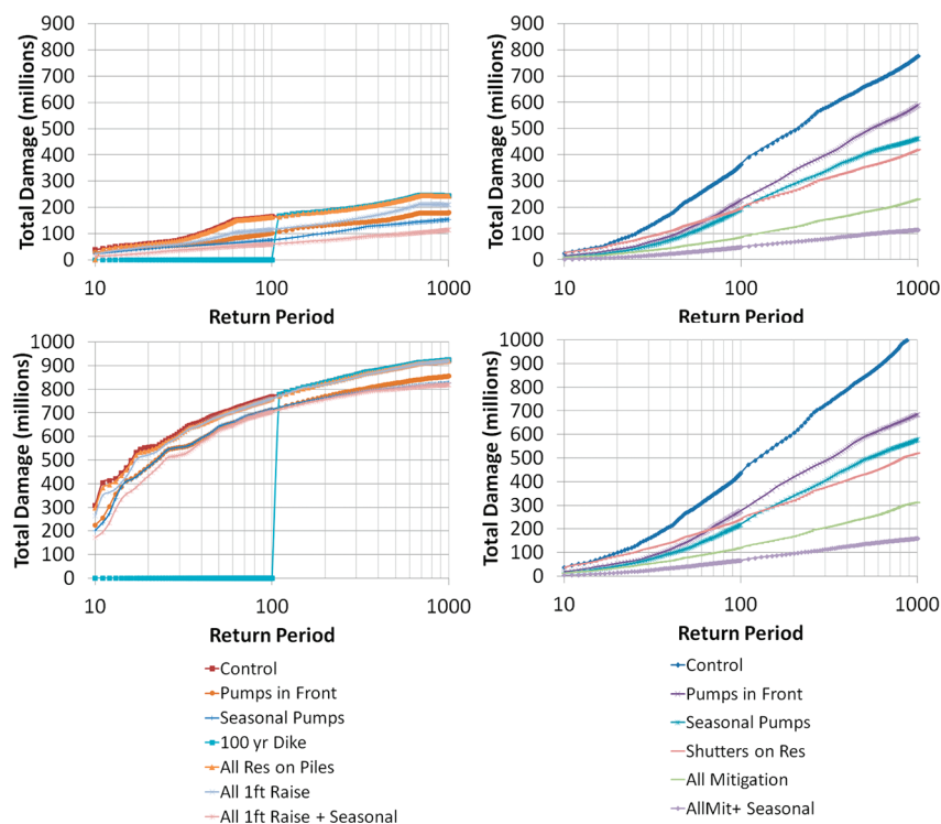
Figure 3. Total damages for scenarios combating storm surge (left) and wind damages (right) for Region 1 (top) and 2 (bottom).
