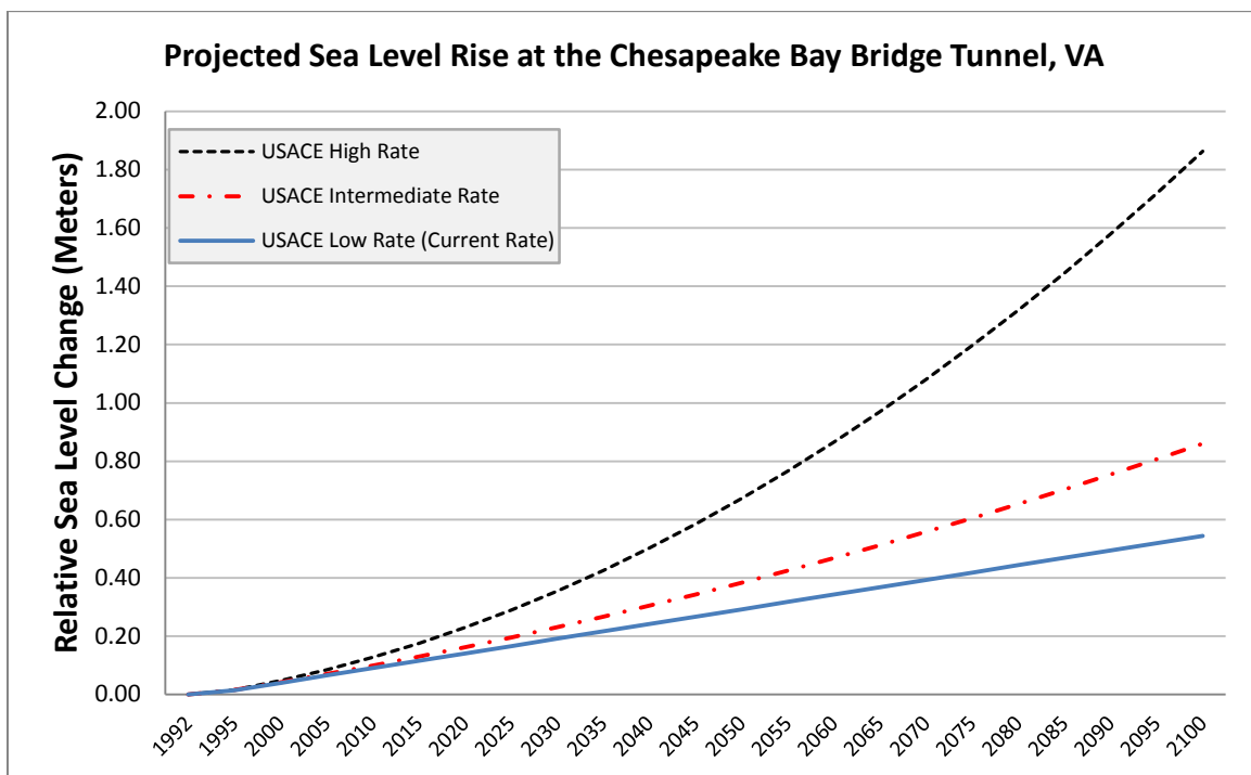
Figure 2: Projected Sea Level Rise, Chesapeake Bay Bridge-Tunnel Station (1992 – 2100)
