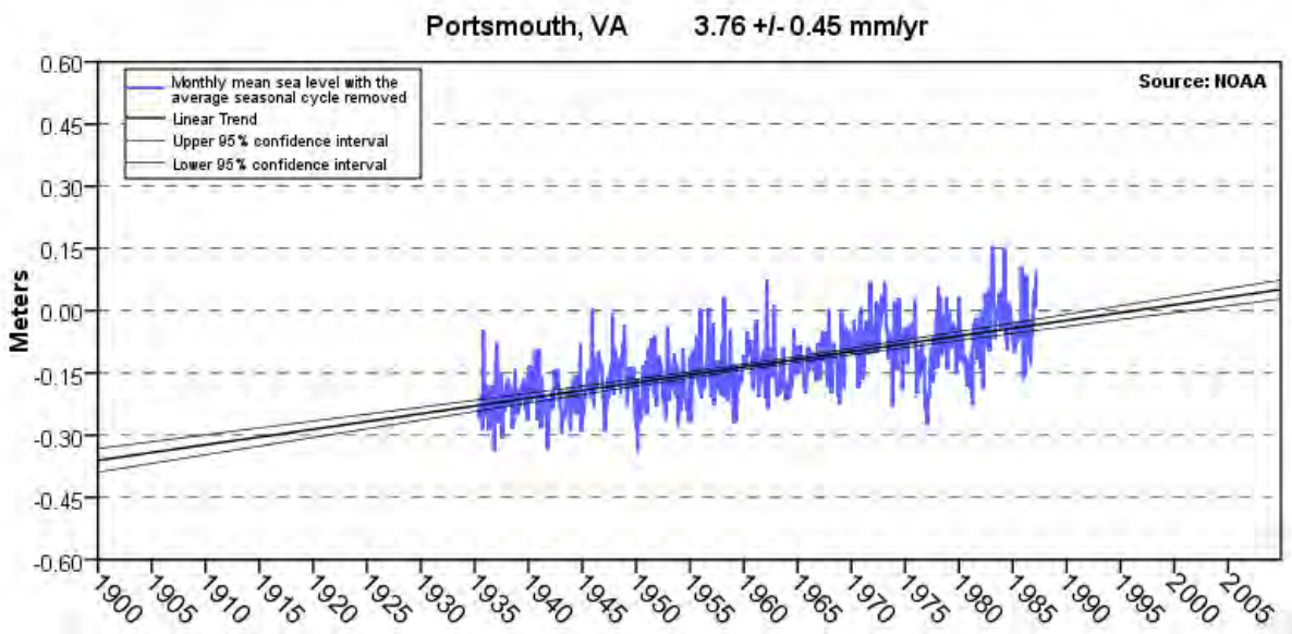
Figure 7: Mean Sea Level Trend, Portsmouth Station (1935 – 1987)
