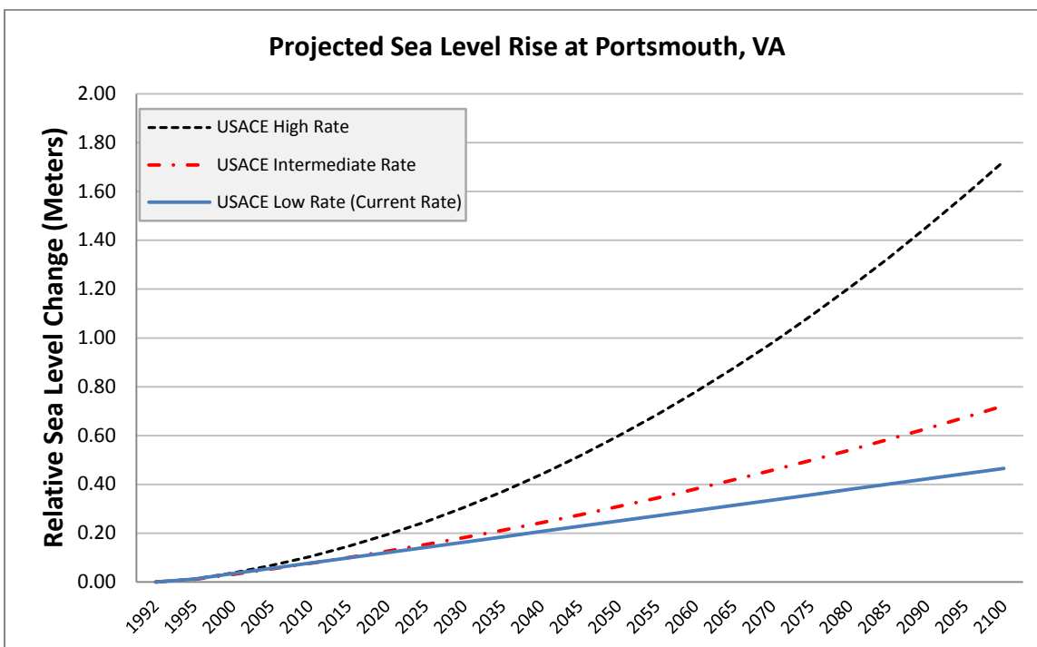
Figure 8: Projected Sea Level Rise, Portsmouth Station (1992 – 2100)
