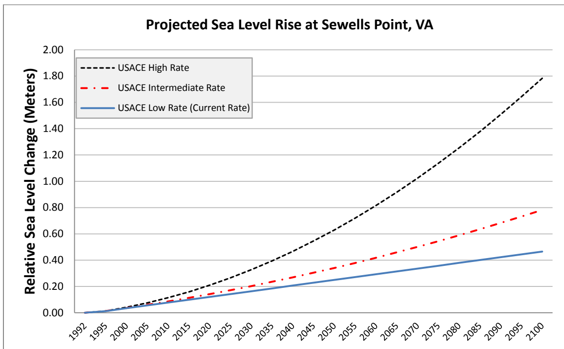
Figure 10: Projected Sea Level Rise, Sewell's Point Station (1992 – 2100)
