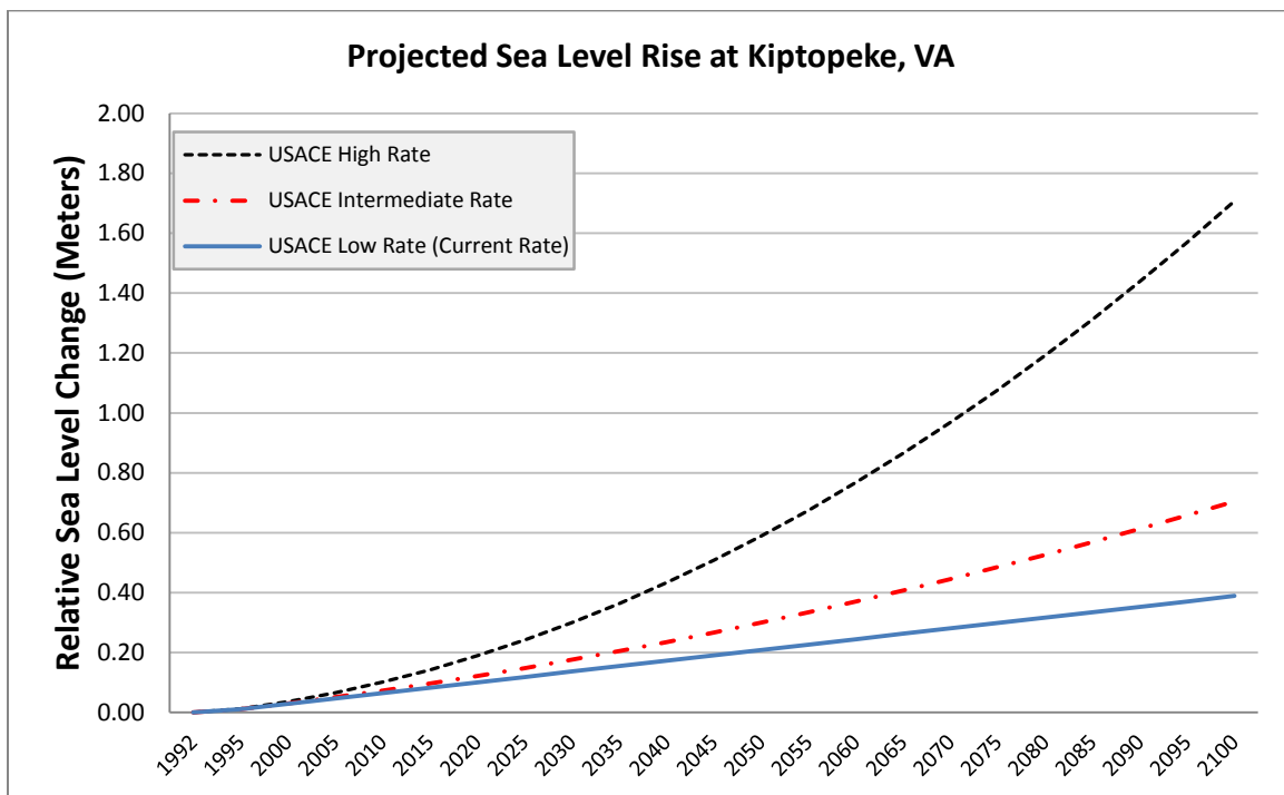
Figure 6: Projected Sea Level Rise, Kiptopeke Station (1992 – 2100)
