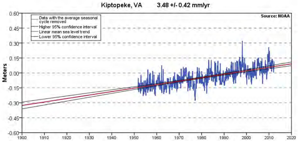
Figure 5: Mean Sea Level Trend, Kiptopeke Station (1951 – 2006)
