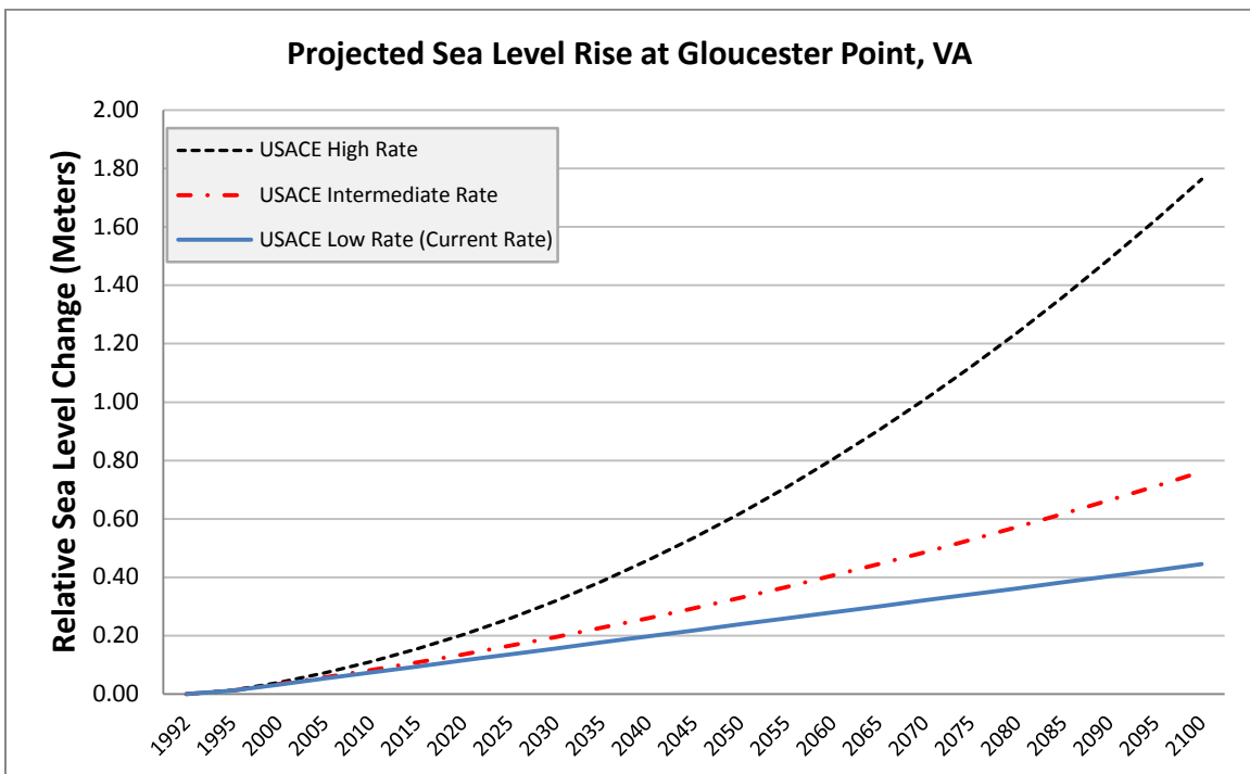
Figure 4: Projected Sea Level Rise, Gloucester Point Station (1992 – 2100)
