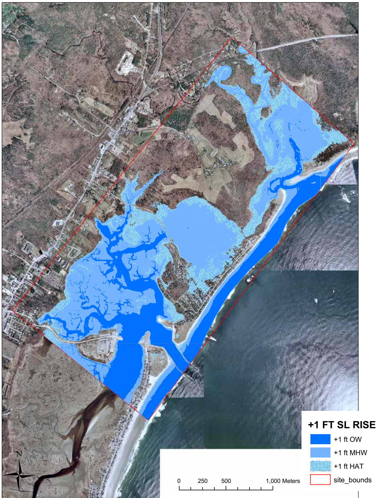
Figure 4. Conditions after a simulated 1 ft static rise in sea level. Most notable are a substantial increase in low marsh area (between OW-MHW) of +14%, and a subsequent decrease in high marsh (between MHW-HAT) of -12% of the study area. There is also a loss of -4% of the upland areas from existing conditions. There is only a minimal increase (2%) in open water areas (below 0 m).
