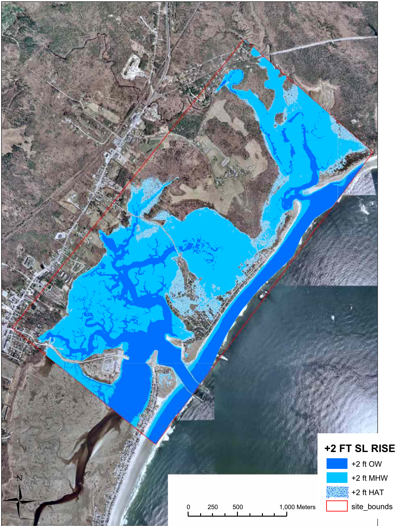
Figure 5. Conditions after a simulated 2 ft static rise in sea level. The low marsh (MHW) continues to overtake the high marsh areas, which is beginning to pinch out along steeper topography. Open water is now 19% of the study area, while low marsh comprises over 33%. Uplands have decreased to about 39% of the study area.
