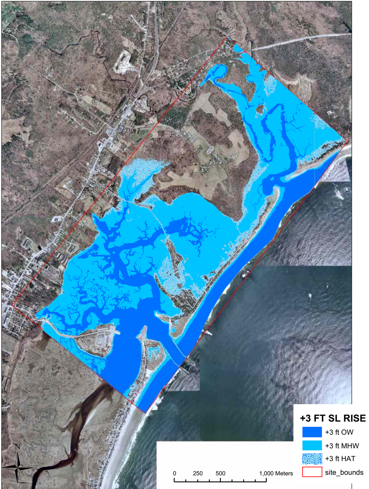
Figure 6. Conditions after a simulated 3 ft static rise in sea level. Overall, low marsh (OW-MHW) has grown over 150% from existing conditions, while the area of high marsh has decreased by 67%. Open water has grown by about 54% from existing conditions, and uplands have lost 25% of their existing conditions area.
