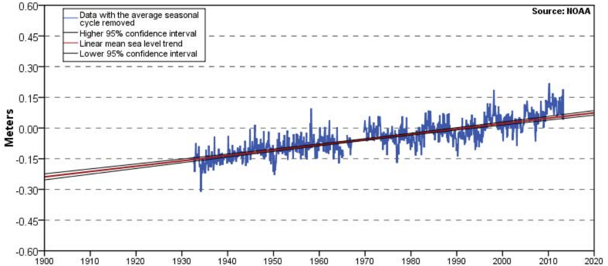
(a) Sea level data for NOAA Woods Hole tide gauge station with linear trend and 95% confidence interval.
