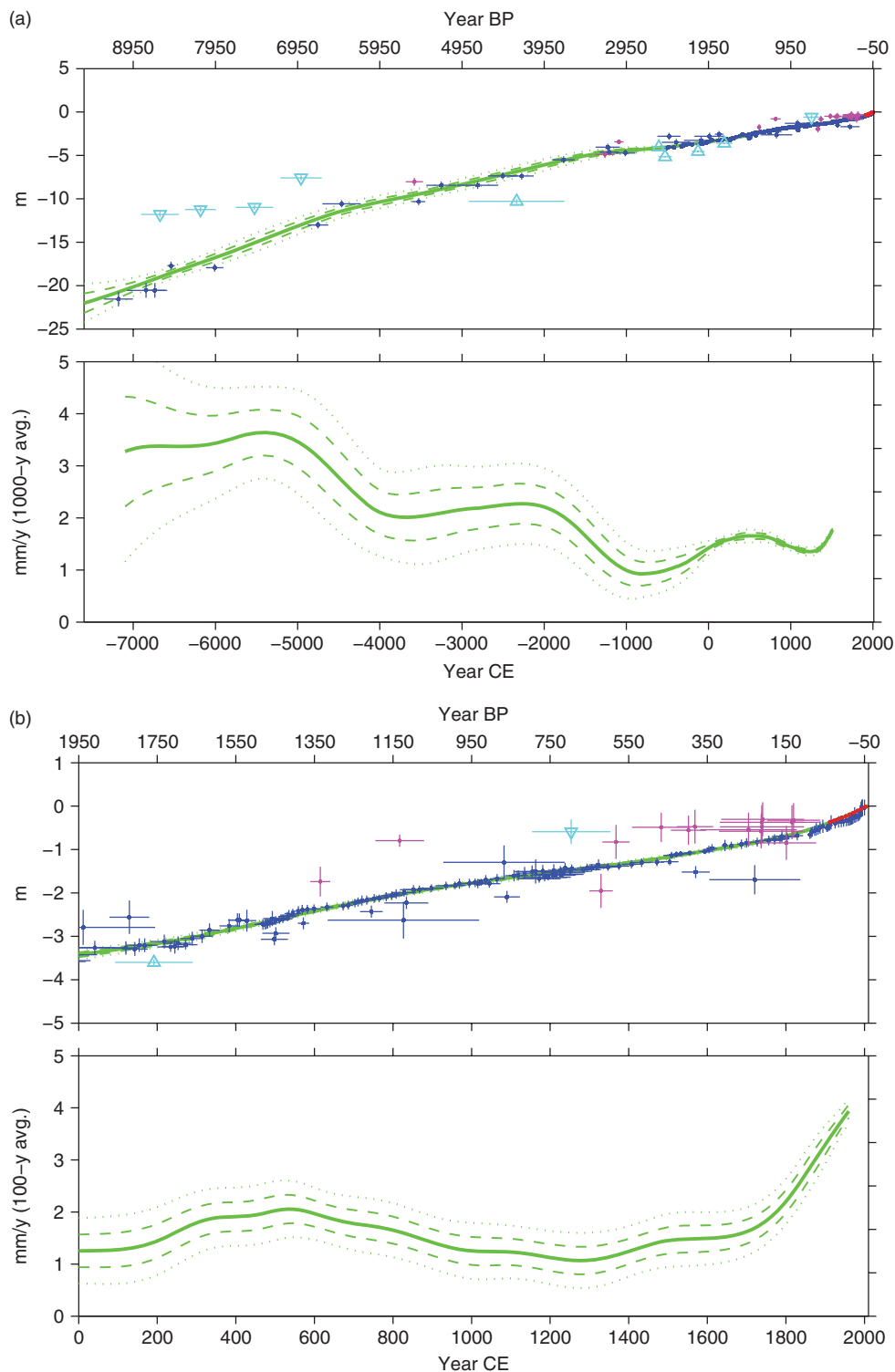
Figure 2. (a) Relative sea-level change over the past 10,000 years in New Jersey using dataset compiled by Horton et al. [2013] and Kemp et al. [2013] for basal (blue) and intercalated (magenta) dates and smoothed Atlantic City tide-gauge data (red); cyan = limiting dates with upward for marine limiting and downward for freshwater limiting, all with 2\sigma error bars. Smoothed line (green) along with 1\sigma (thick dashed line) and 2\sigma (thin dashed line) errors are shown. Bottom plot shows 1000 year average rates of change, plotted at the central year of each 1000 year interval. (b) Enlargement of the Common Era; smoothed line (red) along with 1\sigma (thick dashed line) and 2\sigma (thin dashed line) errors are shown. Bottom plot shows 100 year average rate of change, plotted at the central year of each 1000 year interval. See (a) for description.
