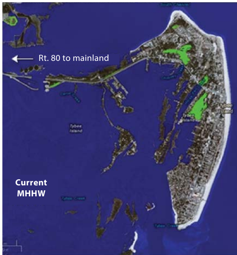
FIGURE 3.1. SEA-LEVEL RISE AND COASTAL FLOODING IMPACTS VIEWER MAPS OF TYBEE ISLAND TODAY (LEFT) AND WITH THREE FEET OF SEA-LEVEL RISE (RIGHT). 39
