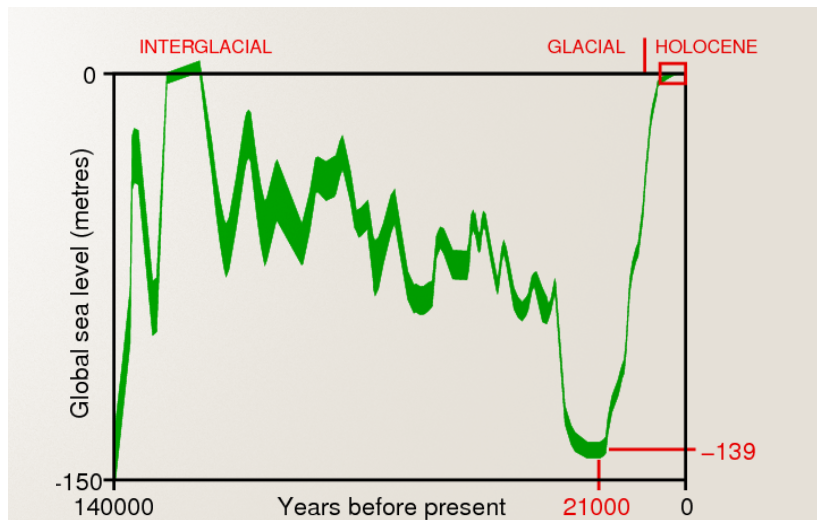
Figure 1. ▲ History of global sea level over the past glacial-interglacial cycle relative to modern-day levels (indicated by the horizontal line at 0 on the graph).
