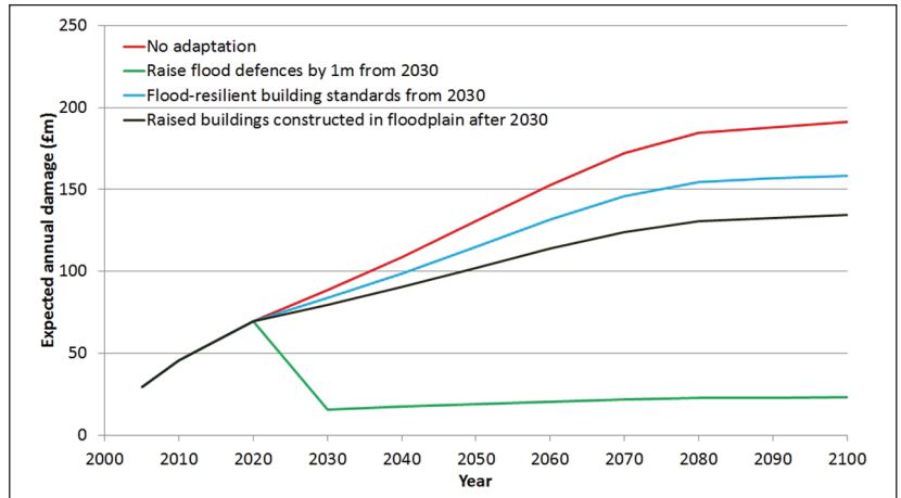
FIGURE 3 Expected annual damage from flooding for the “estuary development” scenario under the UKCP09 medium climate change scenario over time, and the damage reduction benefits of a number of adaptation options implemented in 2030.
