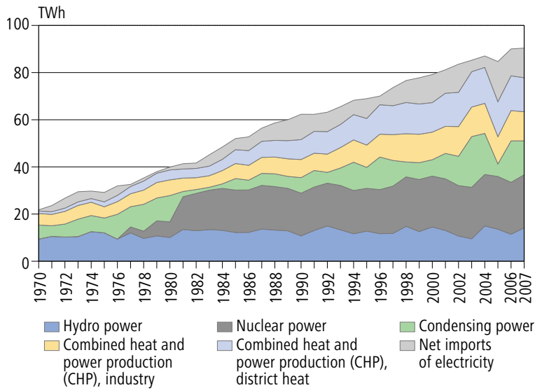
Figure 2.10 Electricity supply by production mode, 1970–2007
