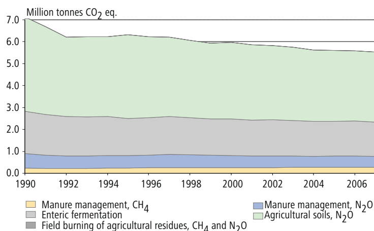
Figure 3.18 Greenhouse gas emissions from agriculture, 1990–2007
