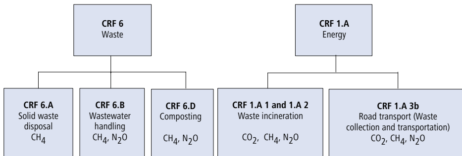
Figure 3.21 Reporting of waste sector emissions in the greenhouse gas inventory
