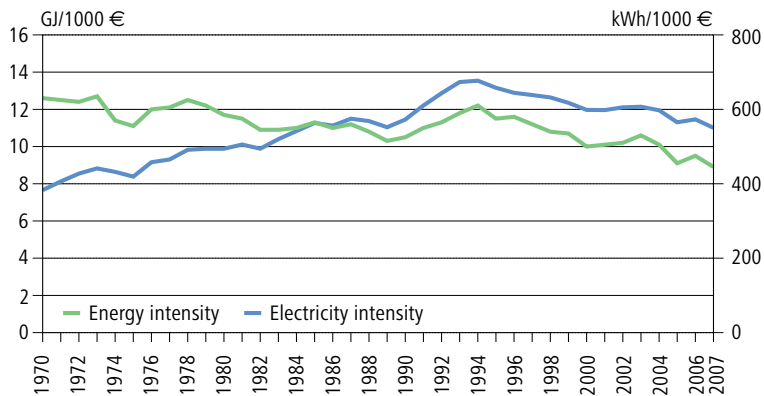
Figure 2.11 Energy and electricity intensity indices, 1970–2007
