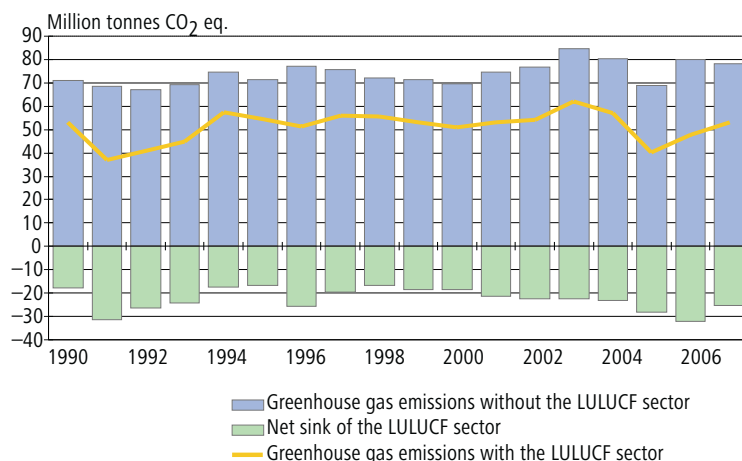
Figure 3.3 Finland's greenhouse gas emissions, 1990–2007, excluding the LULUCF sector (blue bars) and including the LULUCF sector (orange line). The green bar shows the net removals in the LULUCF sector.
