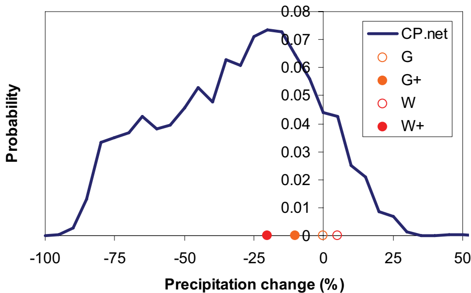
Figure 5.2 Probability density function of summer mean precipitation change (2xCO 2 compared to 1xCO 2 ) over the Netherlands. Also shown are the KNMI scenarios (G, G+, W and W+).
