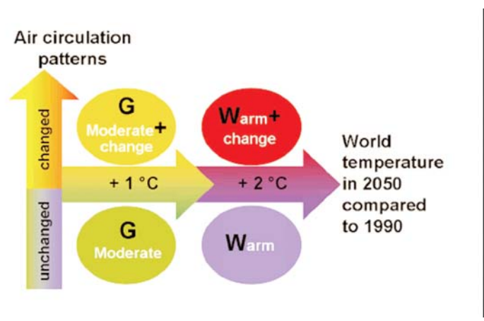
Figure 2.2 Schematic overview of the four KNMI'06 climate scenarios. G=moderate (“gematigd” in Dutch) W=Warm.
