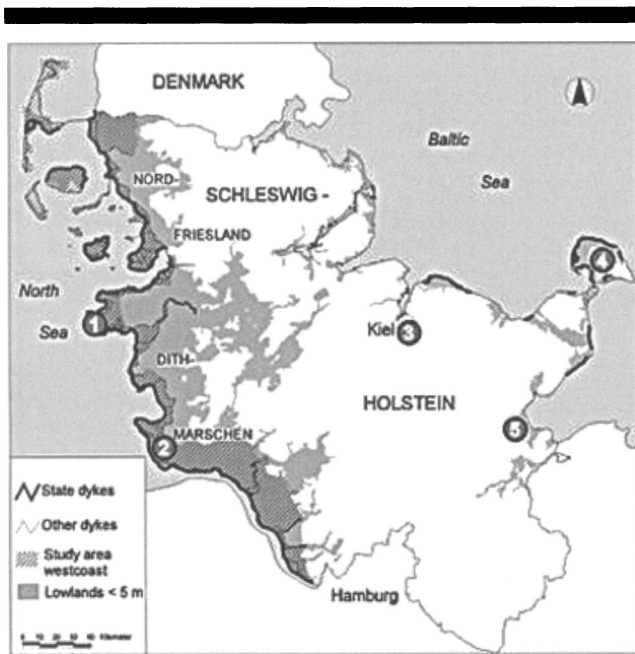
Figure 6. Flood risk areas in the state of Schleswig-Holstein calculated from the meso-scale vulnerability assessment. All shaded areas (below 5-m OD) are potentially flooded lowlands, striped areas are particularly vulnerable in case of dike breakage. Microscale VA: the numbers 1–5 indicate localities where microscale assessments were carried out: (1) St. Peter-Ording: major tourism-oriented community on the North Sea Coast; (2) Kaiser-Wilhelm-Koog: reclaimed farmland secured by dikes, rural character; (3) City of Kiel: largest coastal agglomeration of residents, houses and infrastructure in state; (4) Island of Fehmar: mixed orientation towards agriculture and tourism & recreation; and (5) Timmendorfer Strand: major tourism-oriented community on the Baltic Sea coast.
