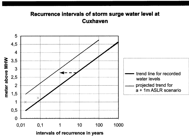
Figure 2. Recurrence intervals of storm surge water levels at Cuxhaven, North Sea coast (data from BSH-statistic and Goennert and Ferk, 1996). An assumed 1-m ASLR would reduce the storm surge interval by at least one order of magnitude.
