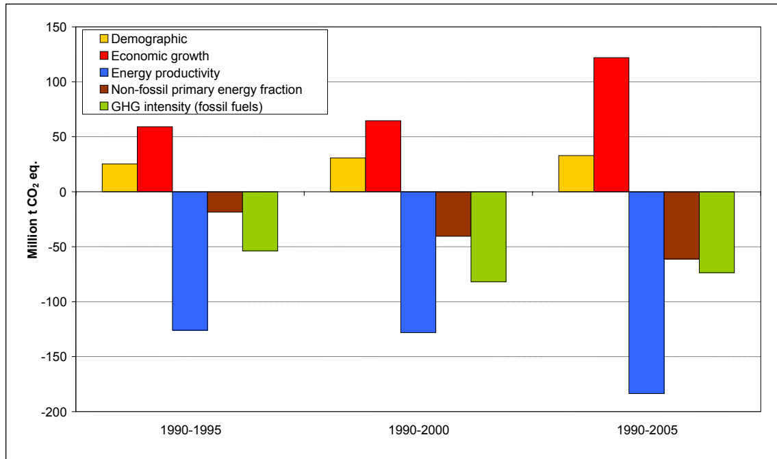
Figure 26 Components of the development of energy-related greenhouse-gas emissions in Germany, 1990-2005
