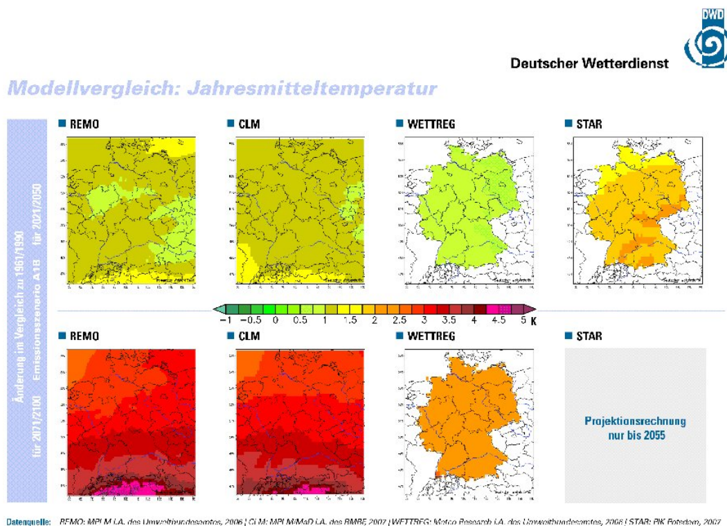
Figure 5: Changes in mean annual temperatures, as predicted by the regional climate models REMO, CLM, WETTREG and STAR, for the A1B emissions scenario in the period 2021-2050 (above) and 2071-2100 (below), in comparison to the corresponding figures for the model-specific control period, 1961-1990
