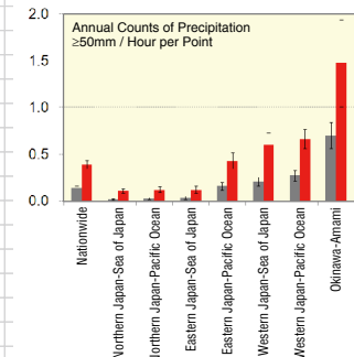
Changes in Annual Counts of Precipitation ≥50mm / Hour by Region
