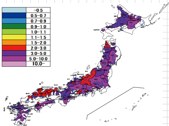
Flooding Magnification Factors by River Basin
