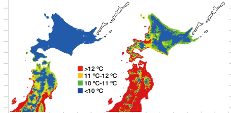
Projected Potential Ranges (Red, Yellow) of the Tiger Mosquito
