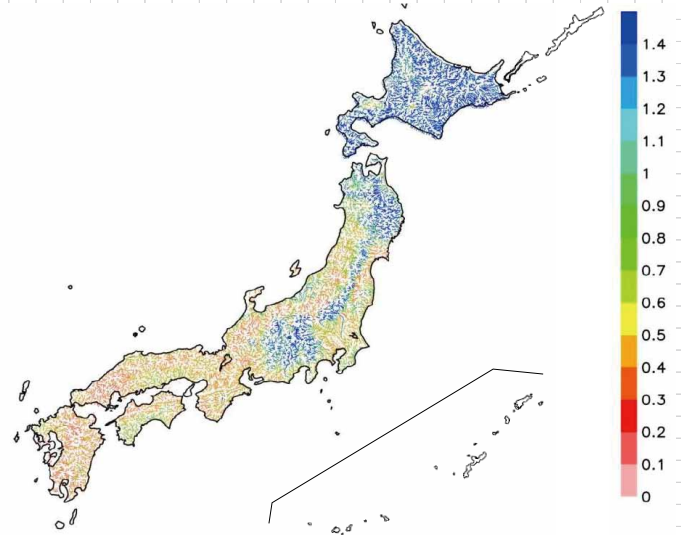
10-year return period Drought-time change (End of the 21st Century)
