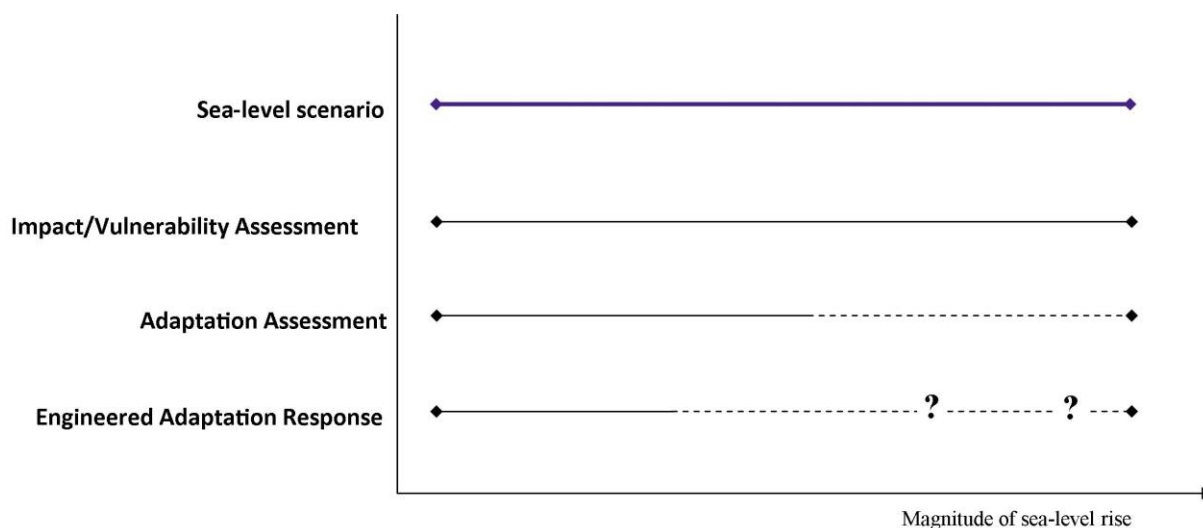
Figure 8: Possible relationship between sea-level scenarios, impact and adaptation.
